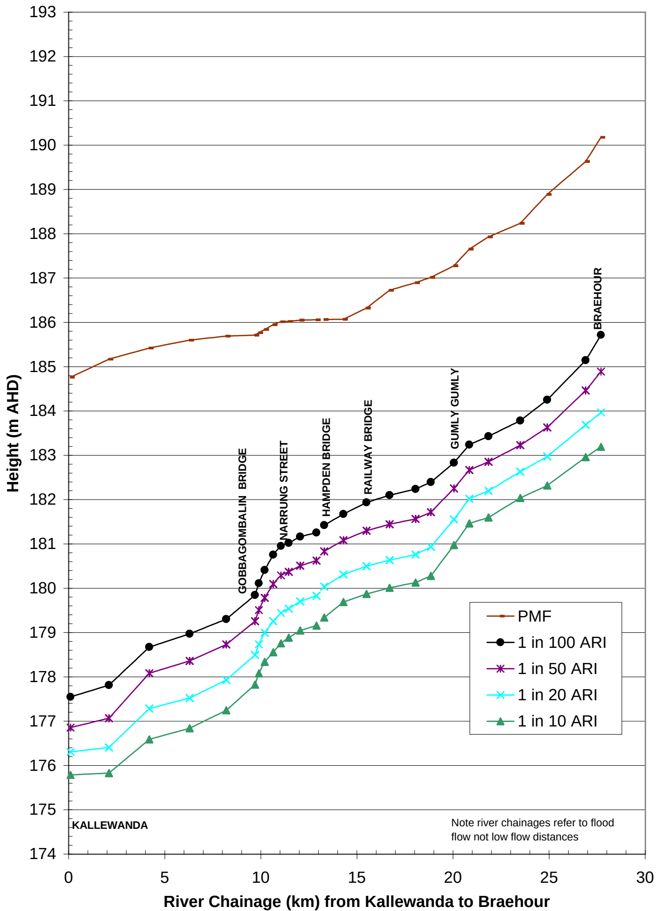
FIGURE 25 PEAK HEIGHT PROFILES DESIGN FLOOD EVENTS
