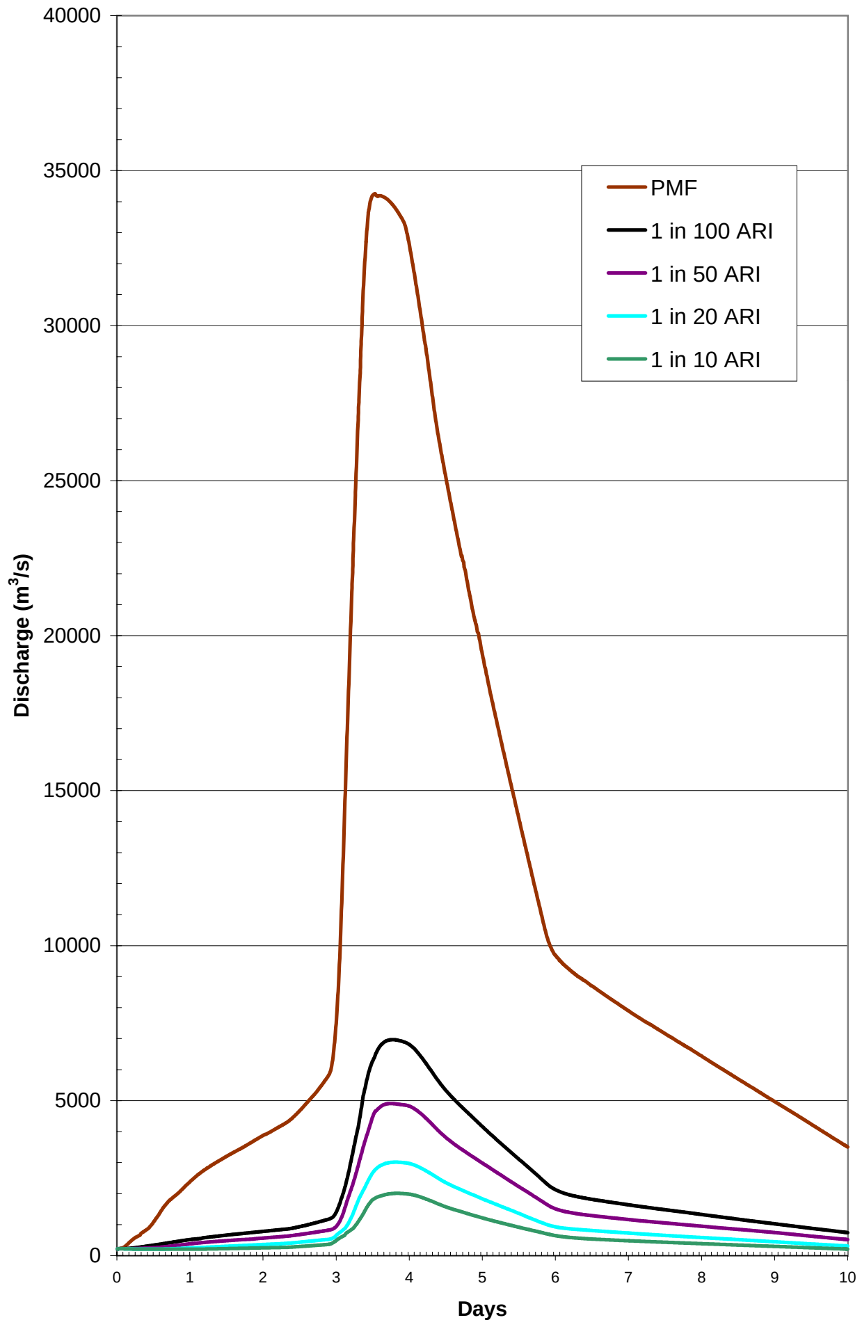
FIGURE 23 DESIGN DISCHARGE HYDROGRAPHS HAMPDEN BRIDGE
