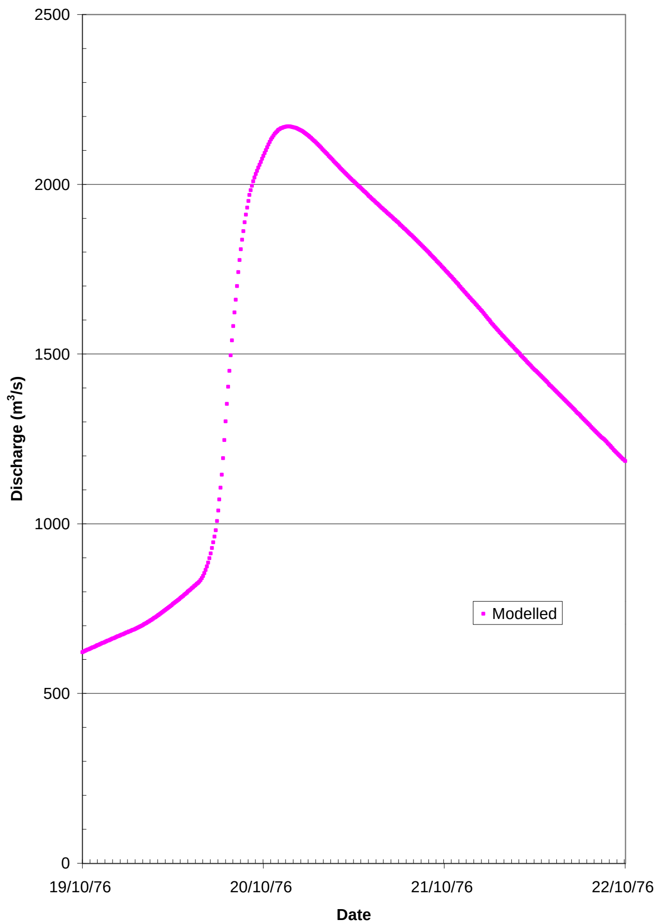
FIGURE 21 DISCHARGE HYDROGRAPH HAMPDEN BRIDGE OCTOBER 1976
