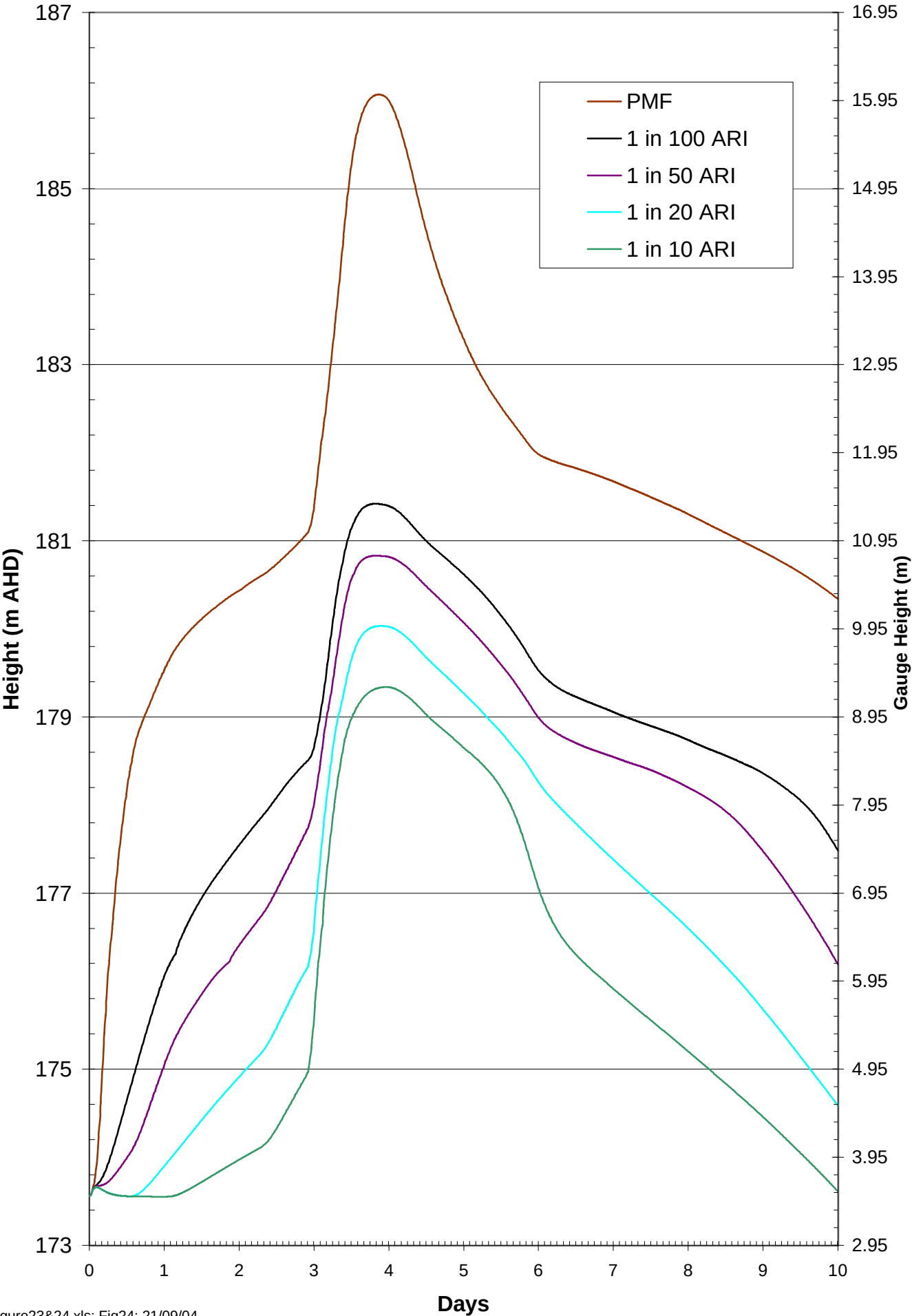
FIGURE 24 DESIGN STAGE HYDROGRAPHS HAMPDEN BRIDGE
