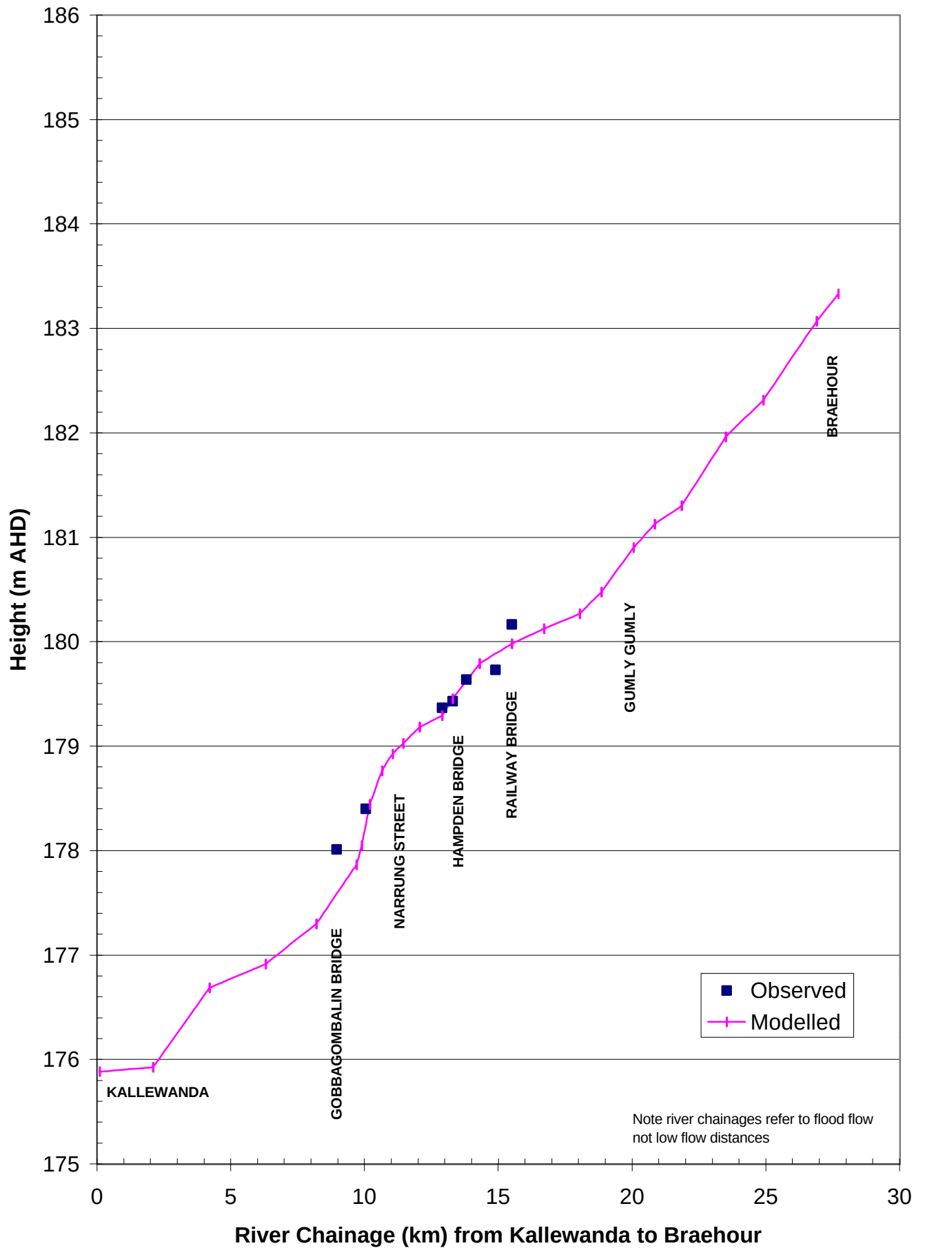
FIGURE 22 PEAK HEIGHT PROFILE OCTOBER 1976
