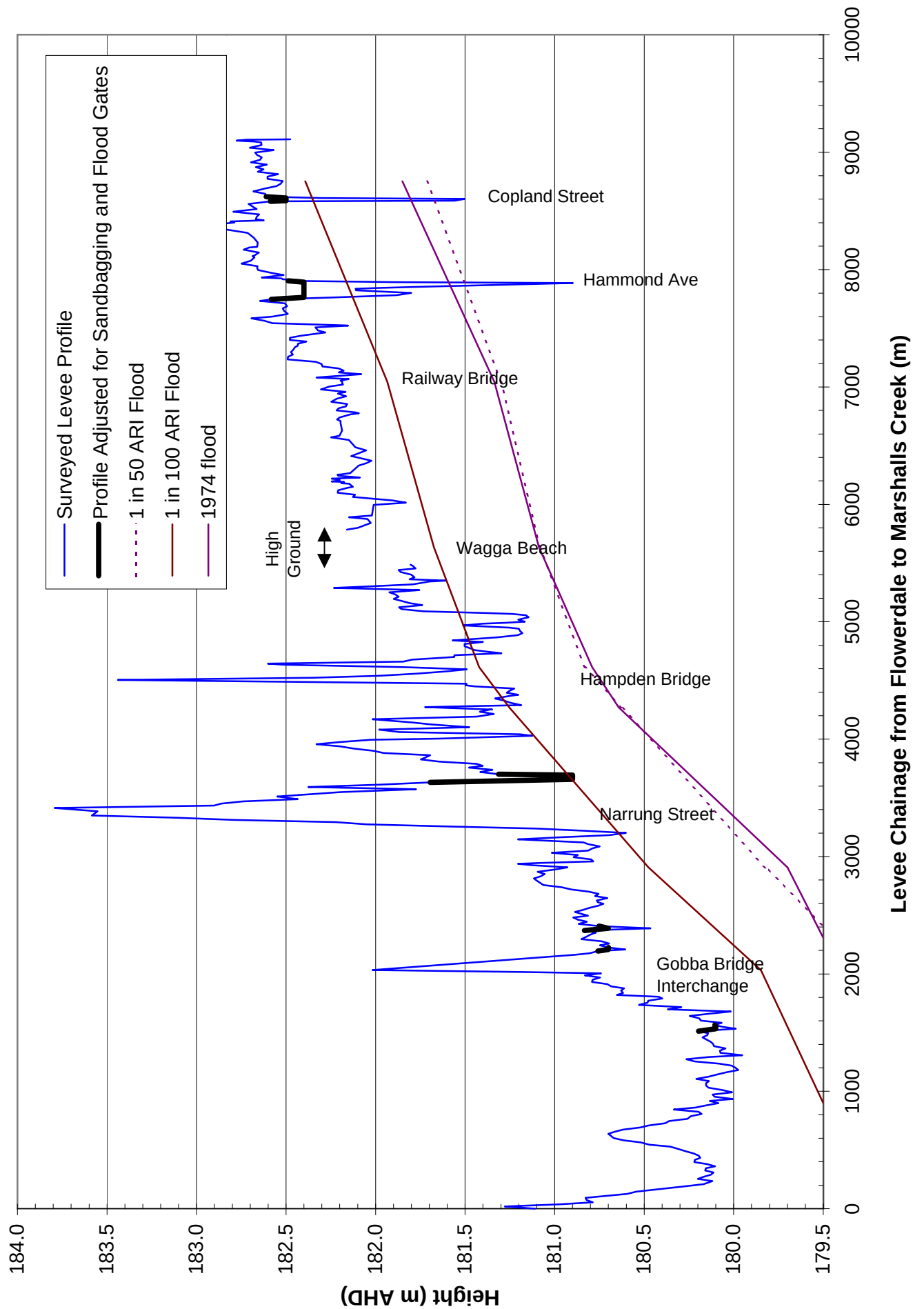
FIGURE 37 MAIN TOWN LEVEE PROFILE DESIGN FLOOD PROFILES
